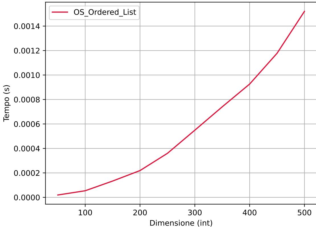
OS Ordered List - Test Casual Selection
